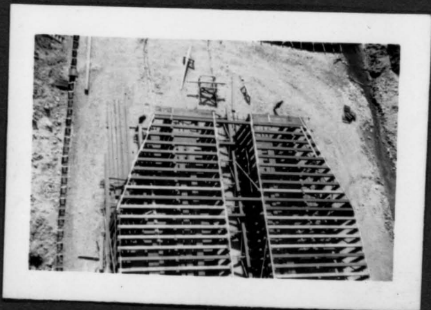
Bow of #4 as seen from the top of the derrick. (115' up).
